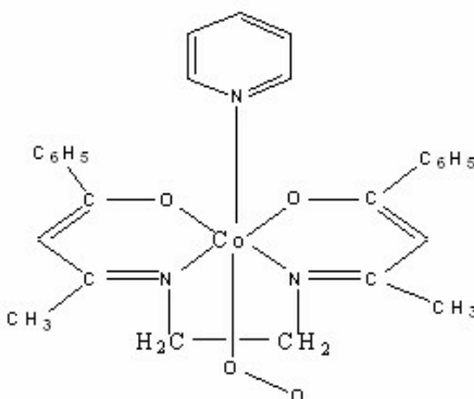
Co(acacen) complex
