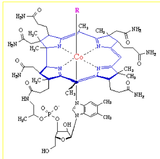
Corrin ring
